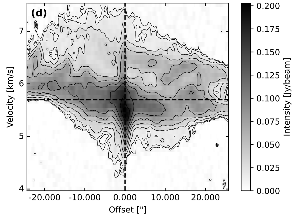
\text{C}^{18}\text{O} (2-1) PV Diagram
